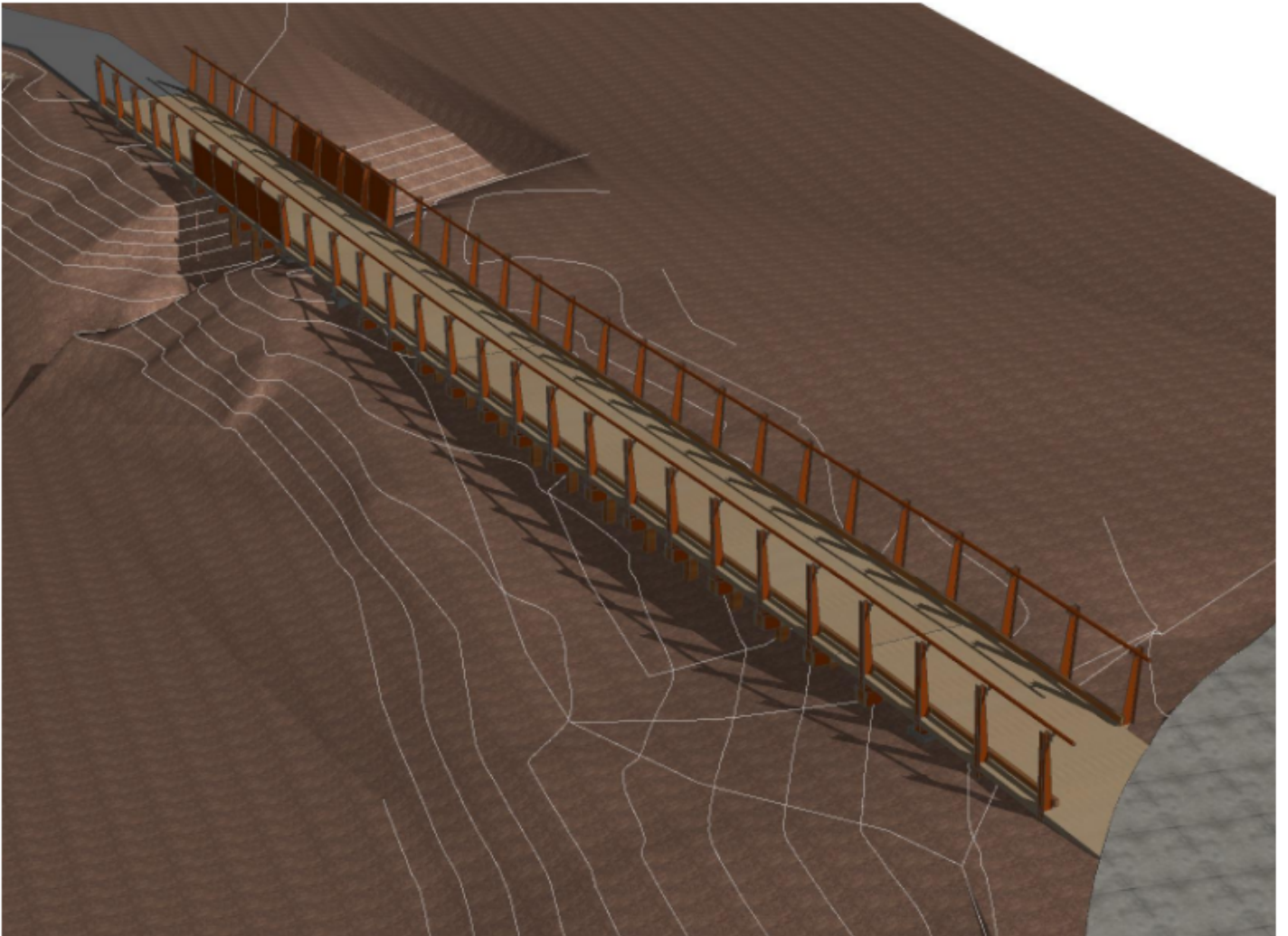
PART A - PERSPECTIVE
